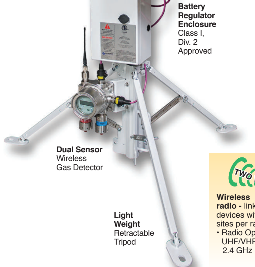
Solar Panel - Class I, Div. 2 Approved
